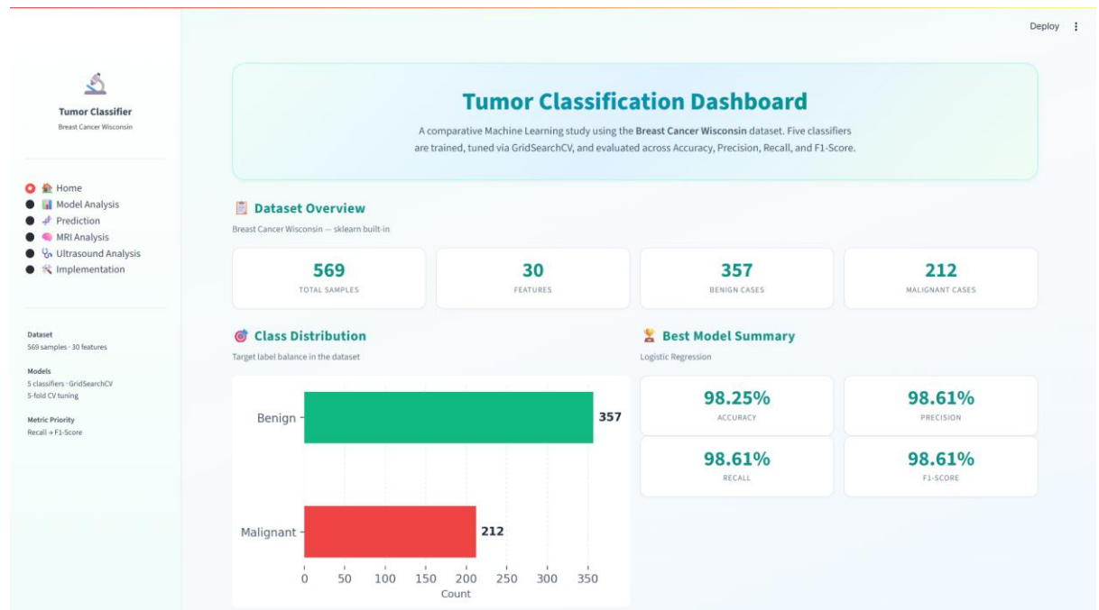
Fig 4.2.1: Dashboard
